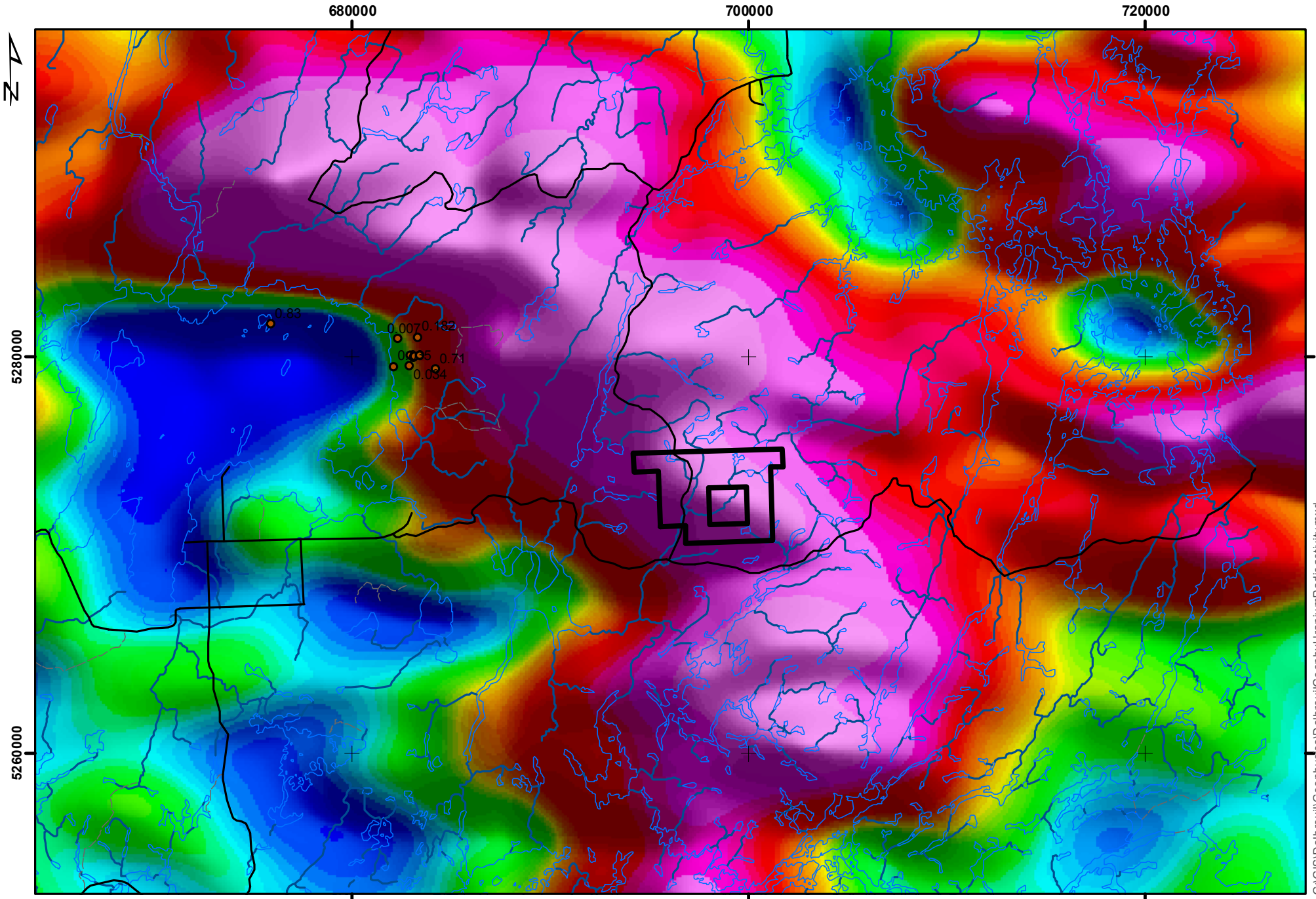
KOOL LAKE RADIOACTIVITY (equivalent uranium, eU) 250 m. grid (From GCC)
